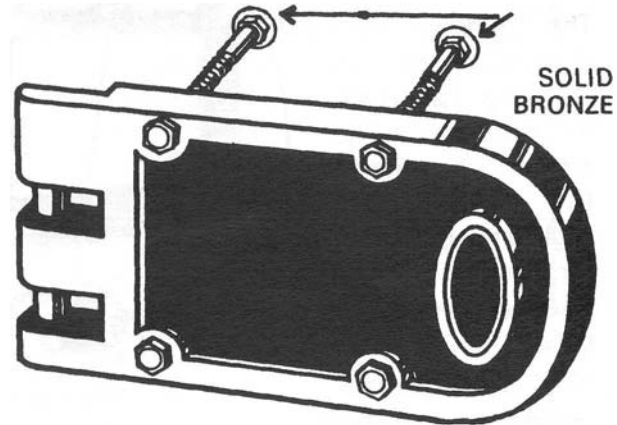
RIM TYPE OR SURFACE LOCK (JIMMY RESISTANT)
